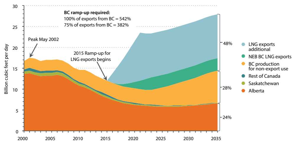
Figure 6: Scenario 1: LNG exports are incremental to NEB reference forecast — five-terminal case, 2000–2035
